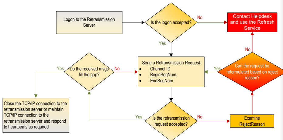
Figure 6: Requesting Dropped Packets
