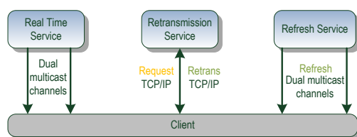
Figure 1: Access to Market Data
