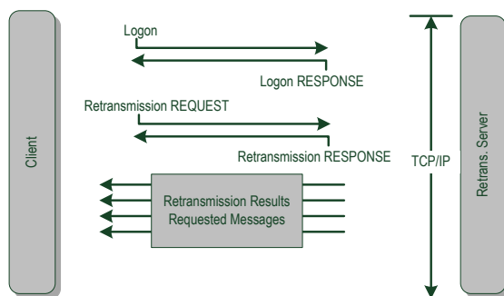
Figure 5: Retransmission Request
