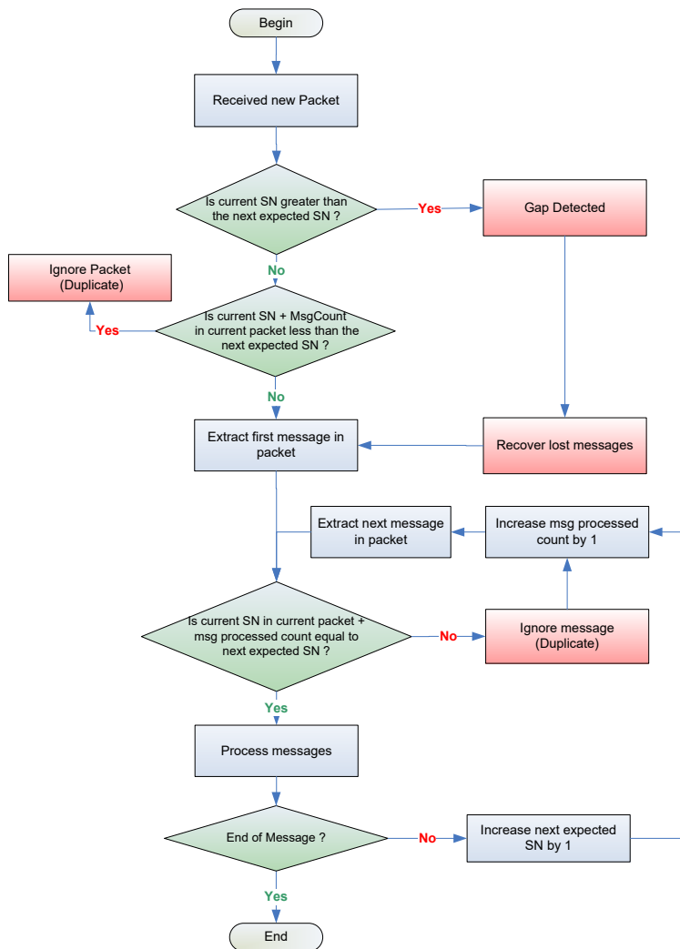
Figure 2: Gap Detection using the Sequence Number (SN)
