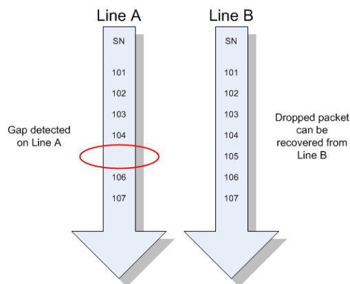
Figure 3 – Detecting Missing Packets
